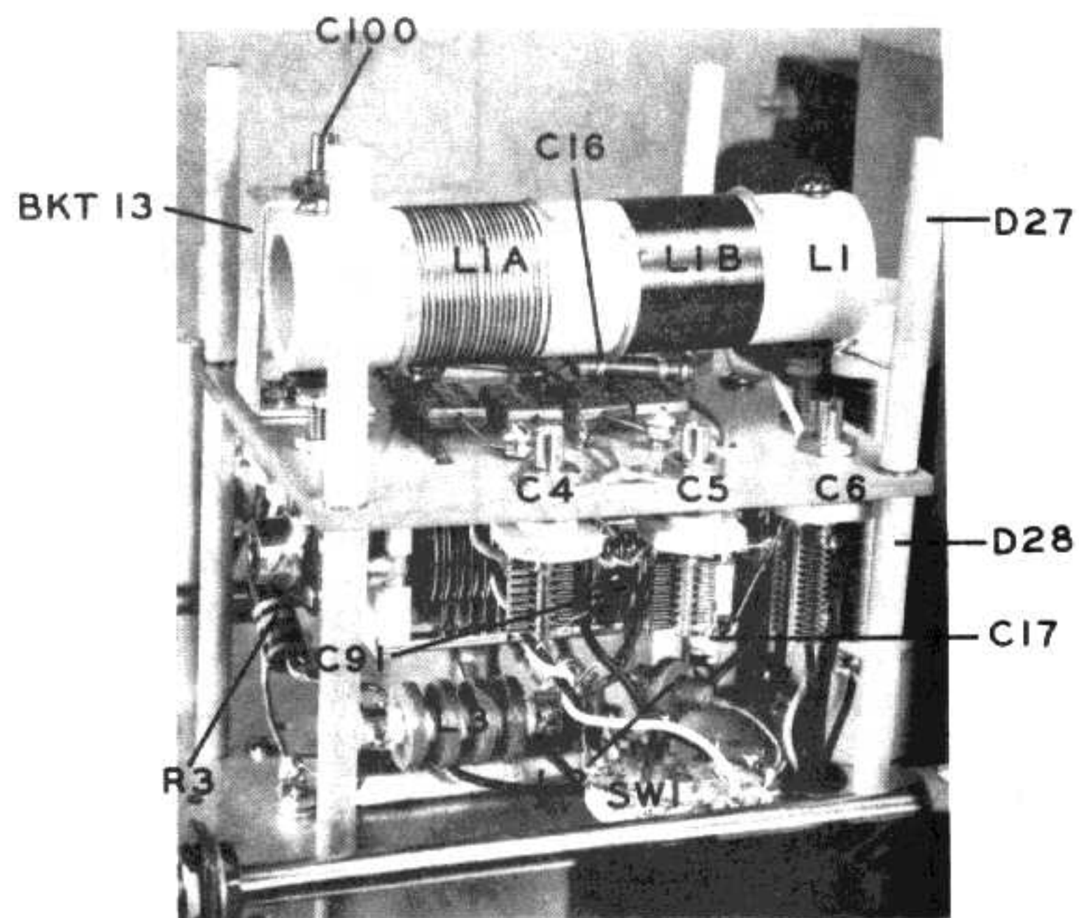
FIGURE 4A VFO RIGHT VIEW
