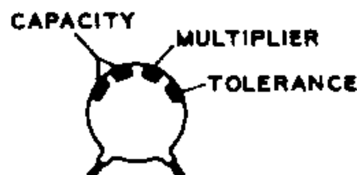
4-DOT DISC CERAMIC RMA CODE
