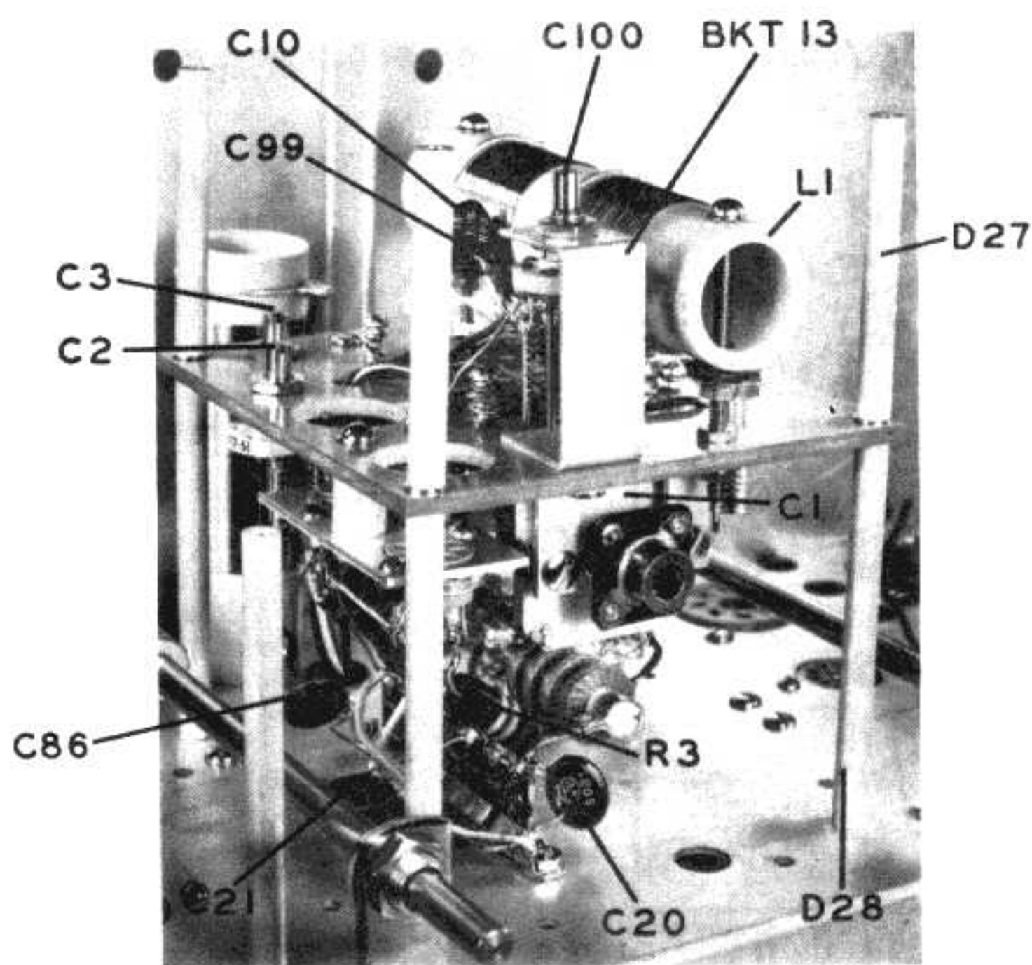
FIGURE 4A VFO LEFT VIEW
