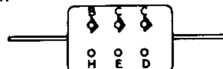
RMA 6-DOT CODE
