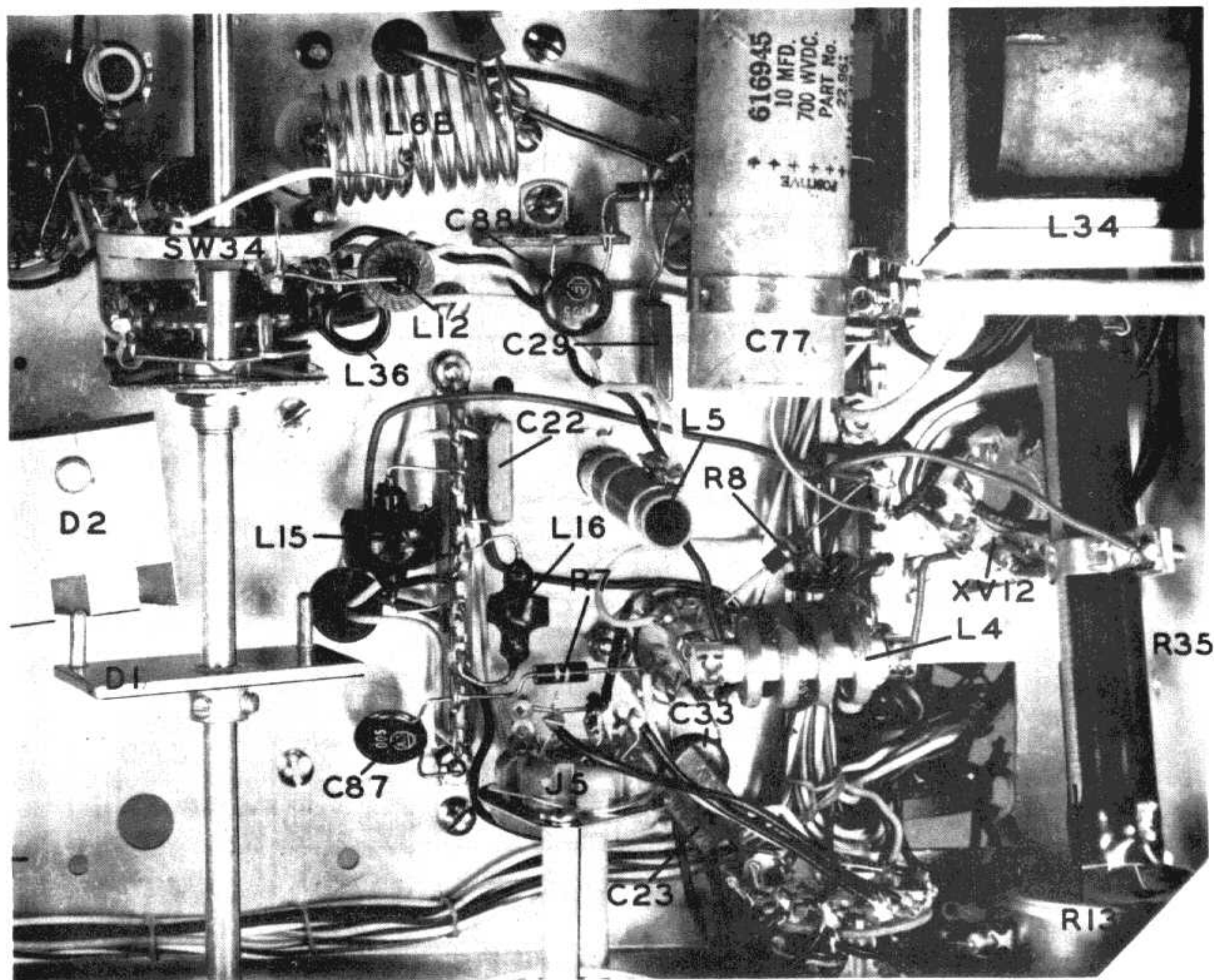
FIGURE 4B-R.F. EXCITER SECTION BOTTOM VIEW
